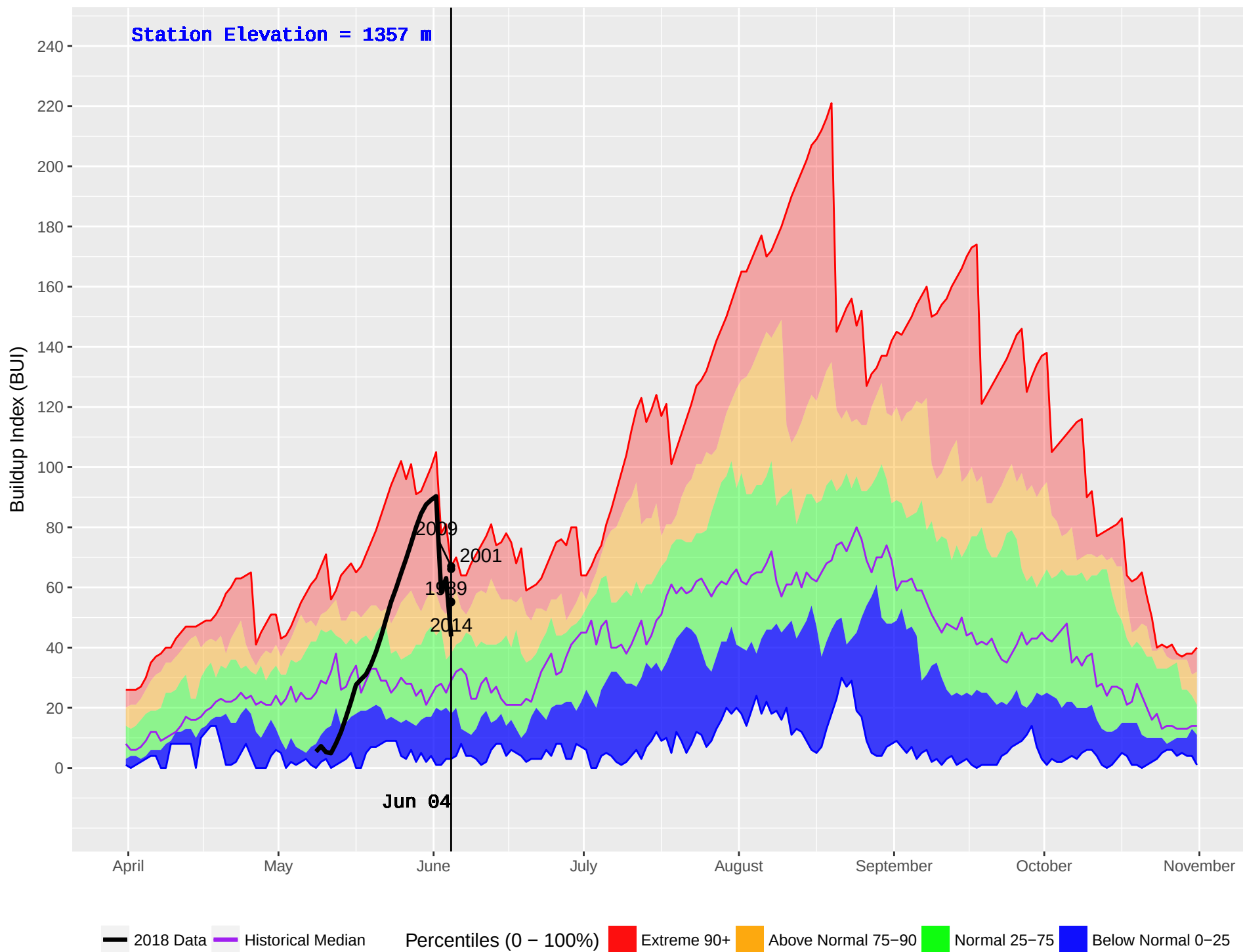
WHITE RIVER (790) : Historical (1989–2016) and Current (2018) Noon Buildup Index (BUI)
