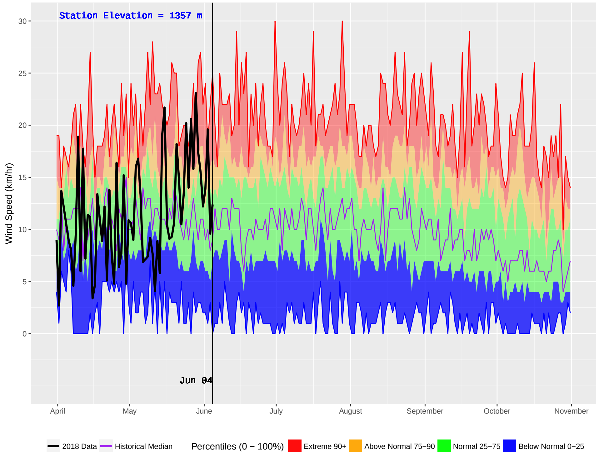
WHITE RIVER (790) : Historical (1989–2016) and Current (2018) Noon Wind Speed
