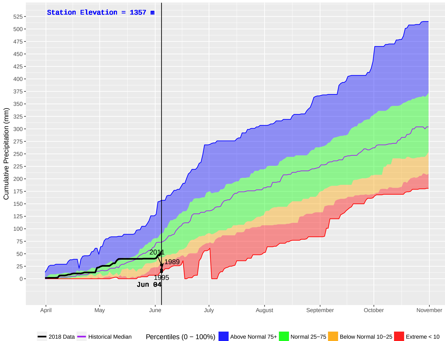
WHITE RIVER (790) : Historical (1989–2016) and Current (2018) Noon Cumulative Precipitation
