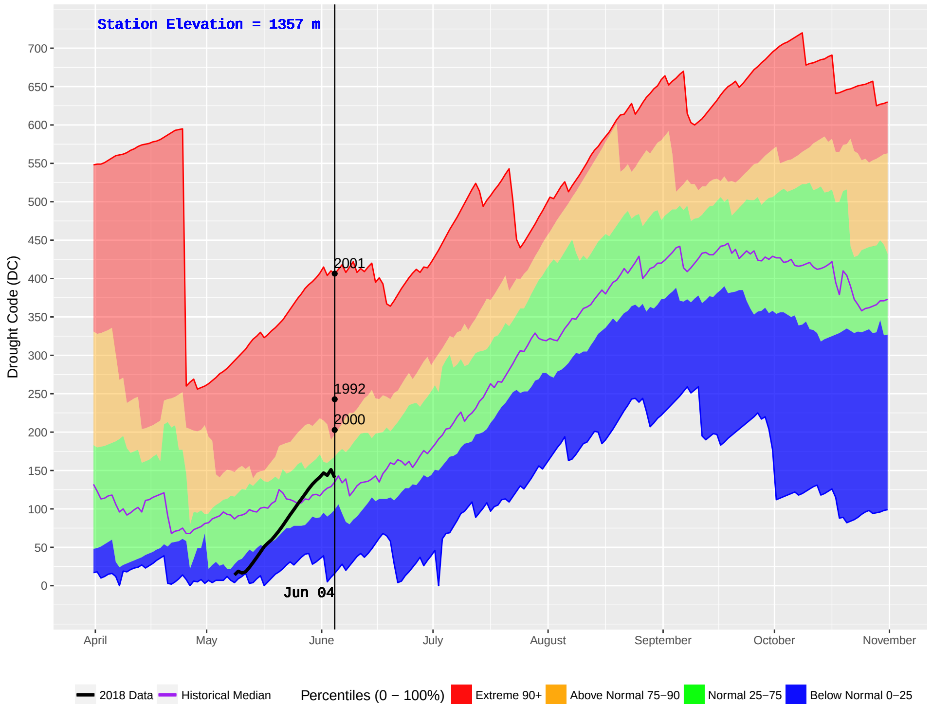
WHITE RIVER (790) : Historical (1989–2016) and Current (2018) Noon Drought Code (DC)
