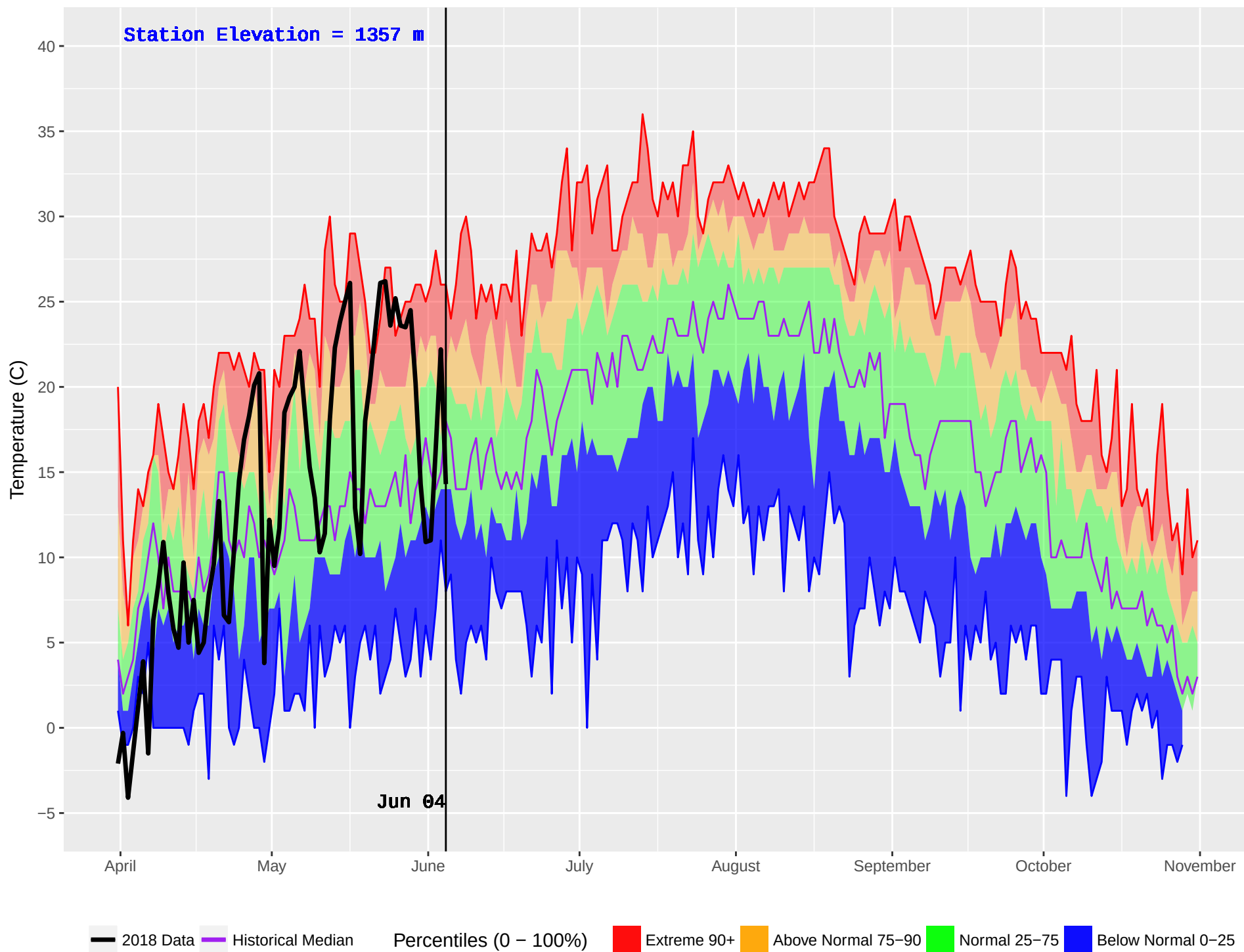
WHITE RIVER (790) : Historical (1989–2016) and Current (2018) Noon Temperature
